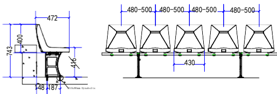
Diamond I - Floor mount
