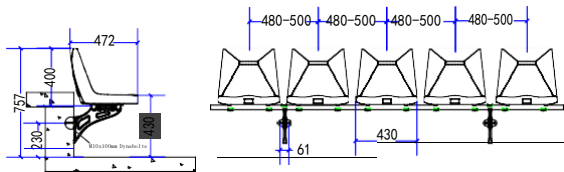
Diamond I - Riser mount
