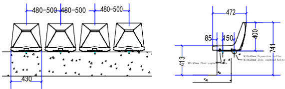
Diamond I - Simple mount
